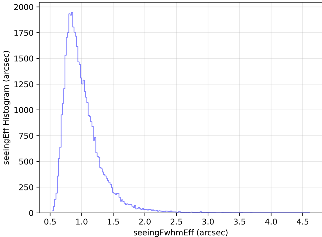
internal_u_expt27_nscale0.9v3.4_10yrs Yr 1 z band: seeingEff Histogram
