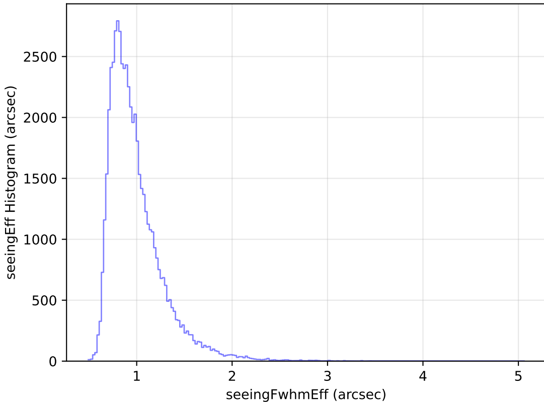
internal_u_expt27_nscale0.9v3.4_10yrs Yr 1 i band: seeingEff Histogram
