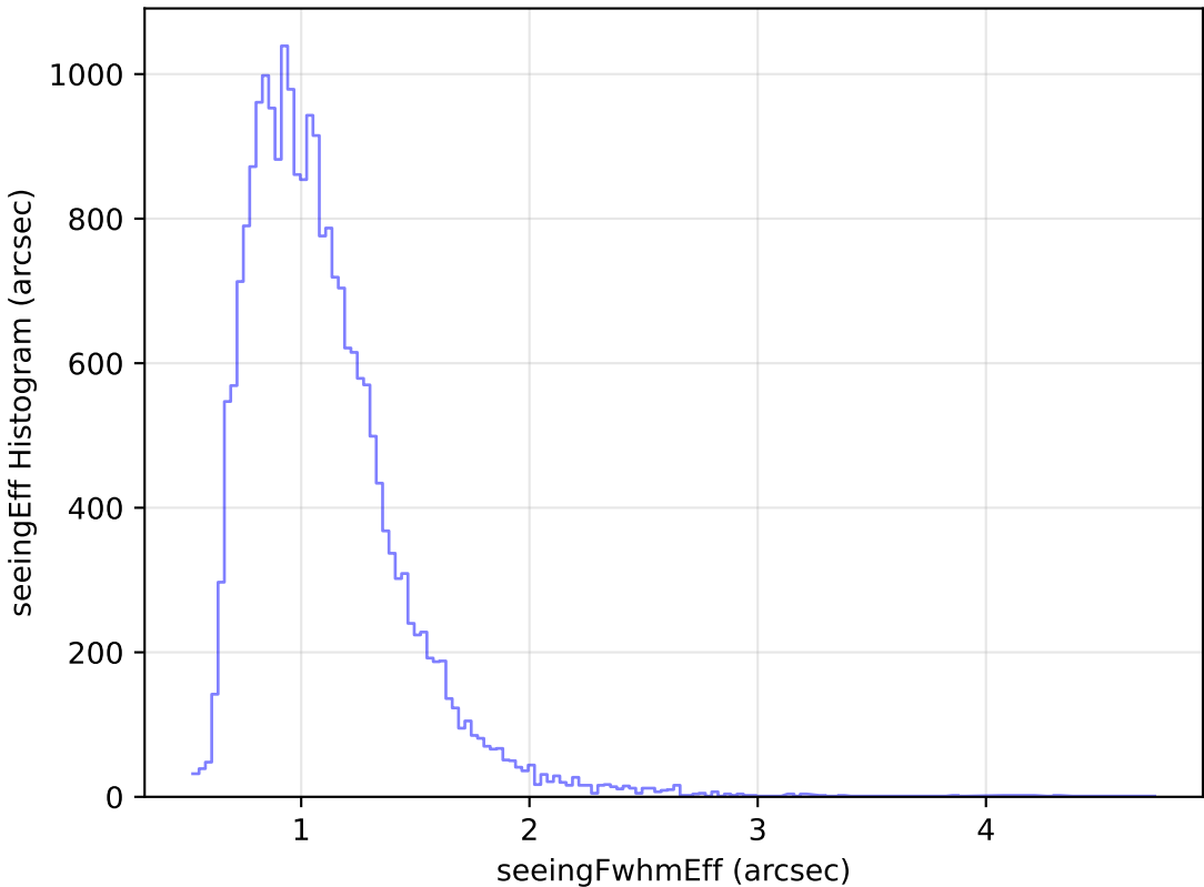
internal_u_expt27_nscale0.9v3.4_10yrs Yr 1 g band: seeingEff Histogram
