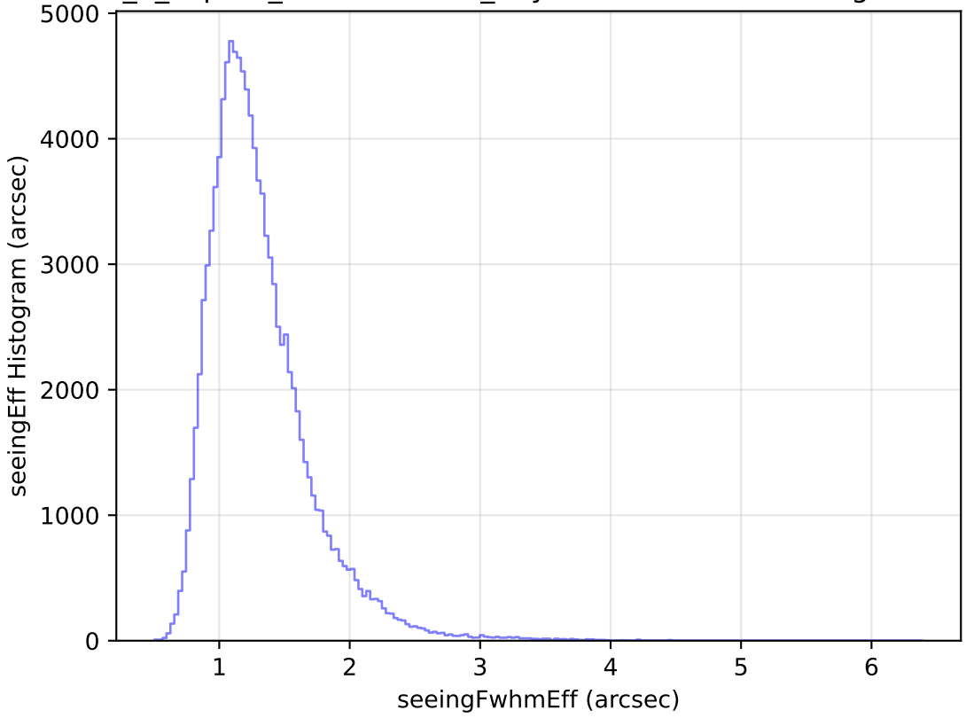
internal_u_expt27_nscale0.9v3.4_10yrs WFD u band: seeingEff Histogram
