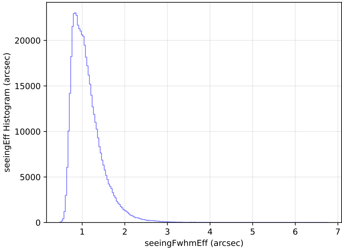
internal_u_expt27_nscale0.9v3.4_10yrs WFD r band: seeingEff Histogram
