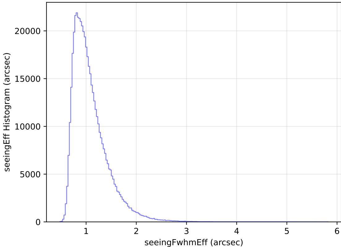
internal_u_expt27_nscale0.9v3.4_10yrs WFD i band: seeingEff Histogram
