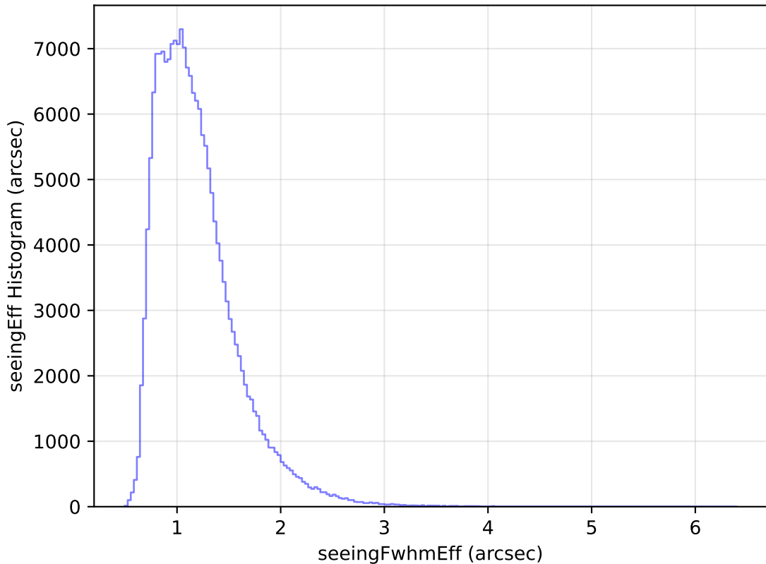
internal_u_expt27_nscale0.9v3.4_10yrs WFD g band: seeingEff Histogram
