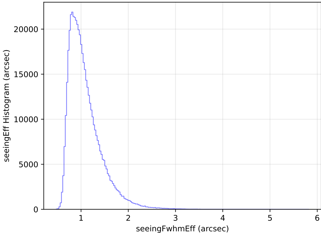
internal_u_expt27_nscale0.9v3.4_10yrs All sky i band: seeingEff Histogram
