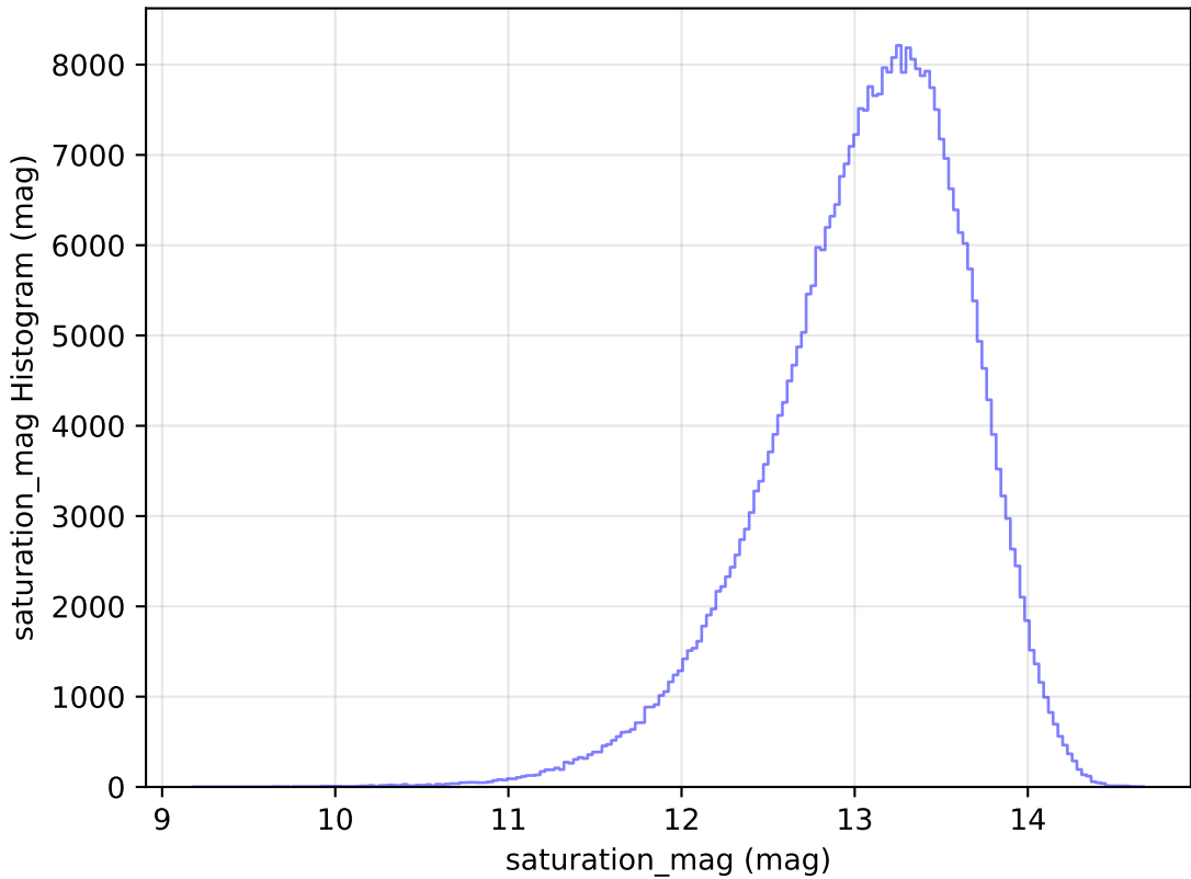
internal_u_expt27_nscale0.9v3.4_10yrs WFD y band: saturation_mag Histogram
