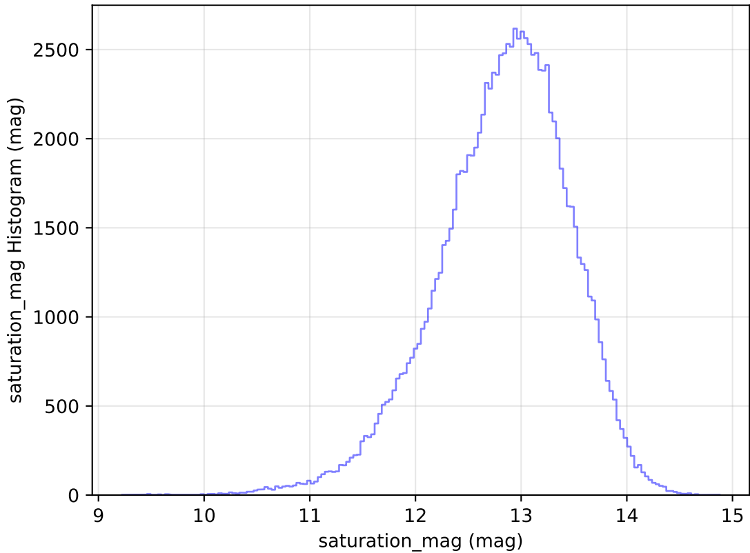
internal_u_expt27_nscale0.9v3.4_10yrs WFD u band: saturation_mag Histogram
