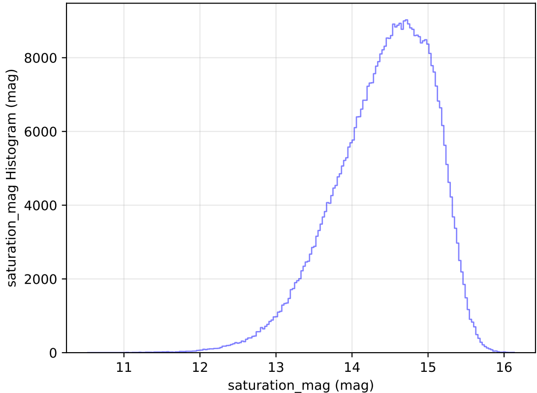
internal_u_expt27_nscale0.9v3.4_10yrs WFD i band: saturation_mag Histogram
