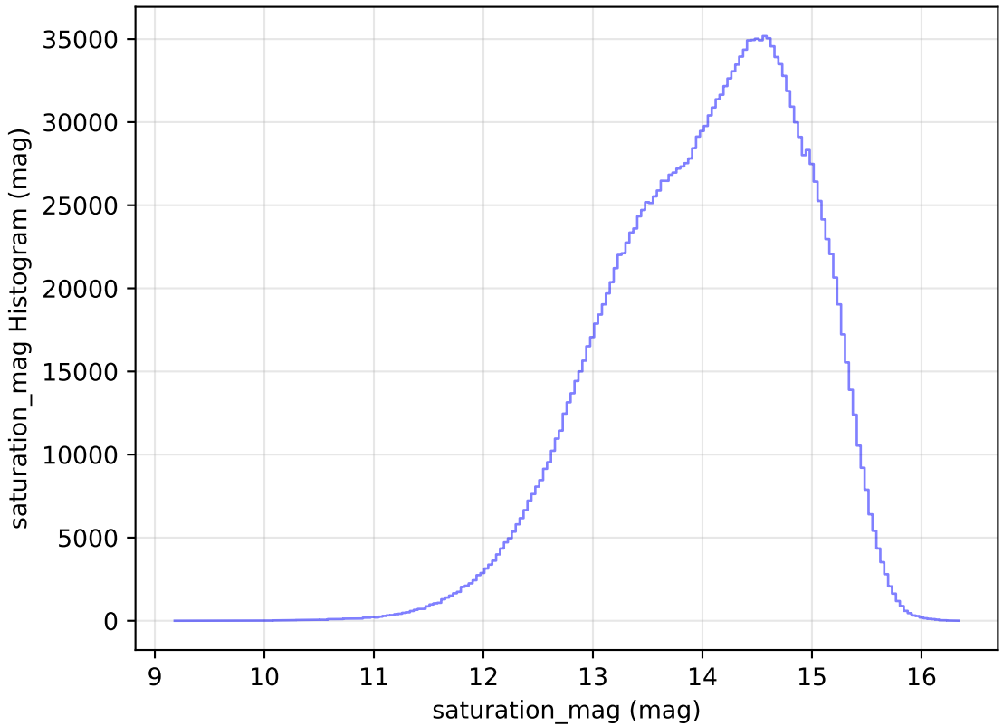
internal_u_expt27_nscale0.9v3.4_10yrs WFD all bands: saturation_mag Histogram
