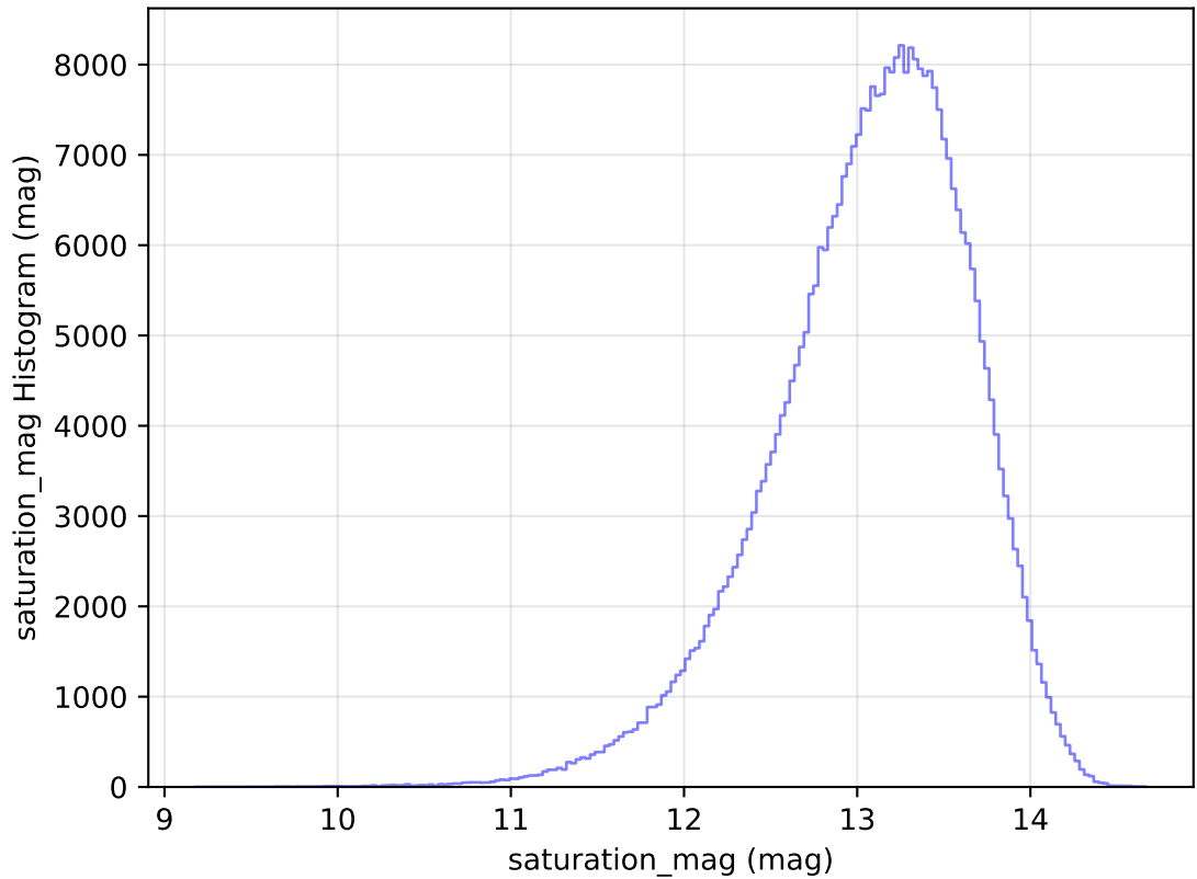
internal_u_expt27_nscale0.9v3.4_10yrs All sky y band: saturation_mag Histogram
