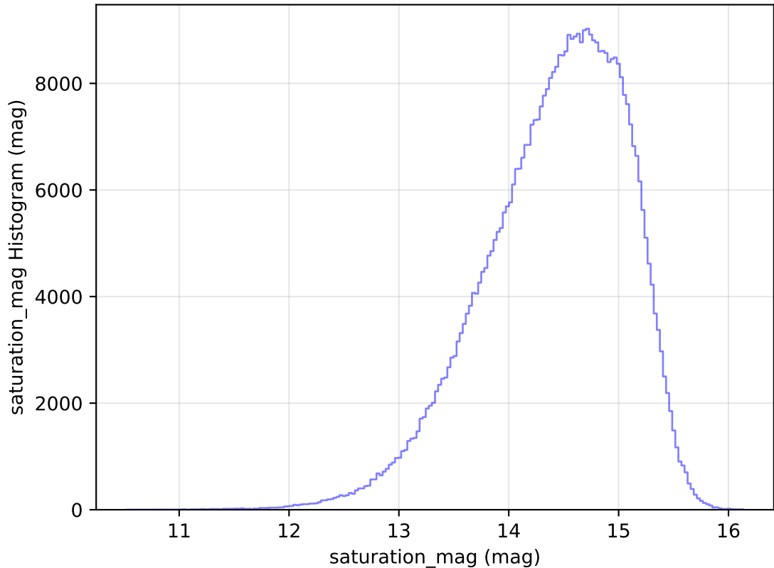
internal_u_expt27_nscale0.9v3.4_10yrs All sky i band: saturation_mag Histogram
