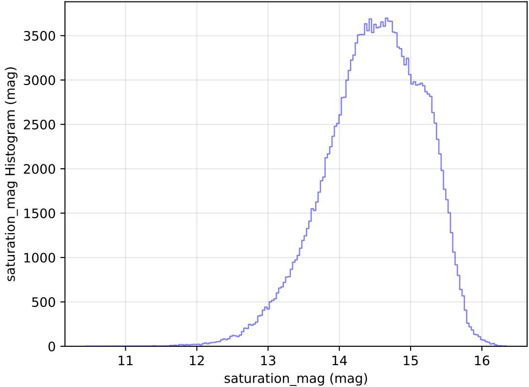
internal_u_expt27_nscale0.9v3.4_10yrs All sky g band: saturation_mag Histogram
