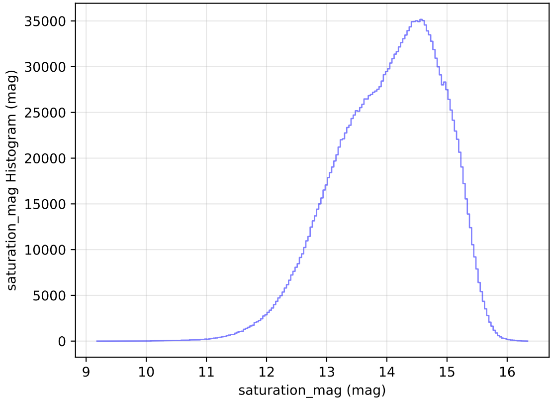
internal_u_expt27_nscale0.9v3.4_10yrs All sky all bands: saturation_mag Histogram
