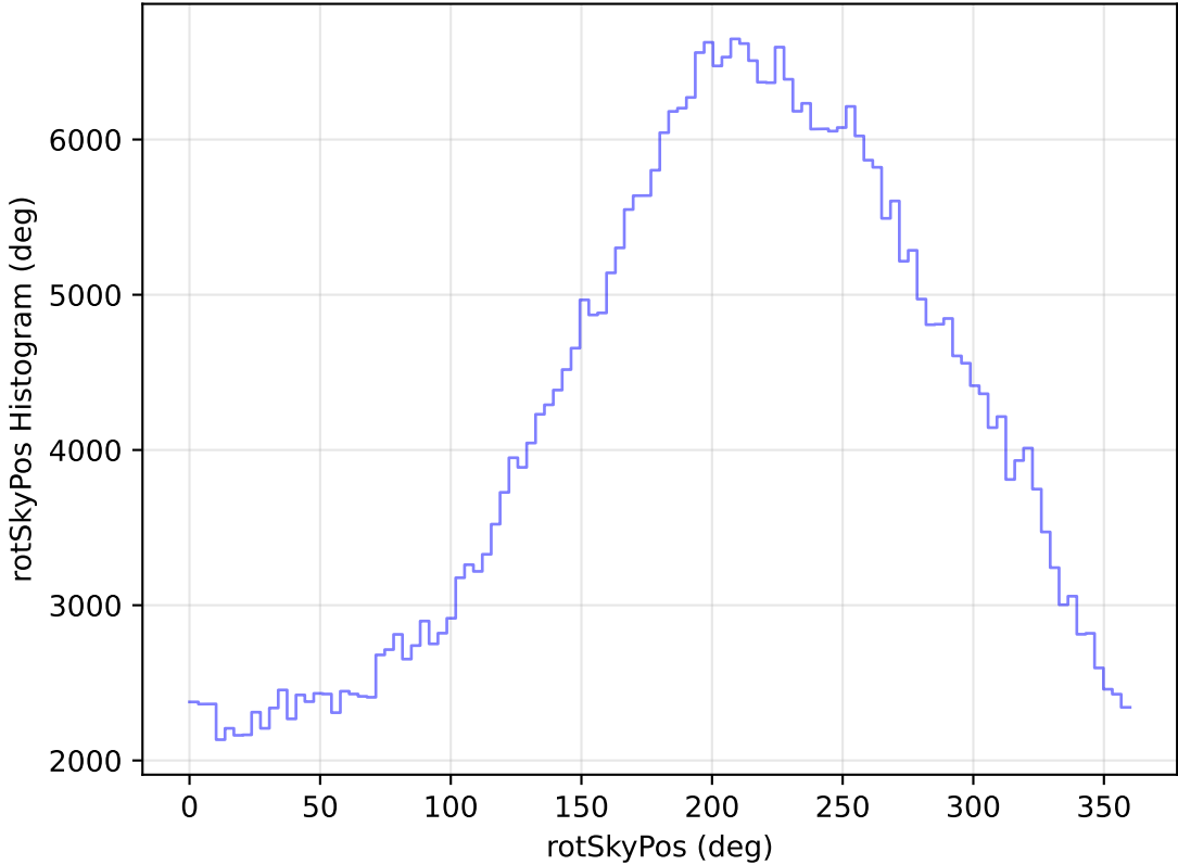
internal_u_expt27_nscale0.9v3.4_10yrs WFD z band: rotSkyPos Histogram
