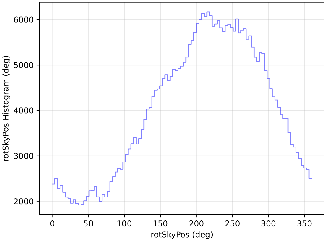
internal_u_expt27_nscale0.9v3.4_10yrs WFD y band: rotSkyPos Histogram
