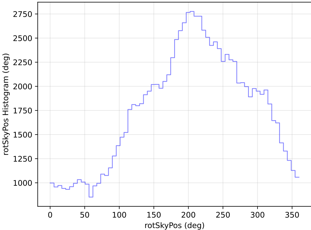
internal_u_expt27_nscale0.9v3.4_10yrs WFD u band: rotSkyPos Histogram
