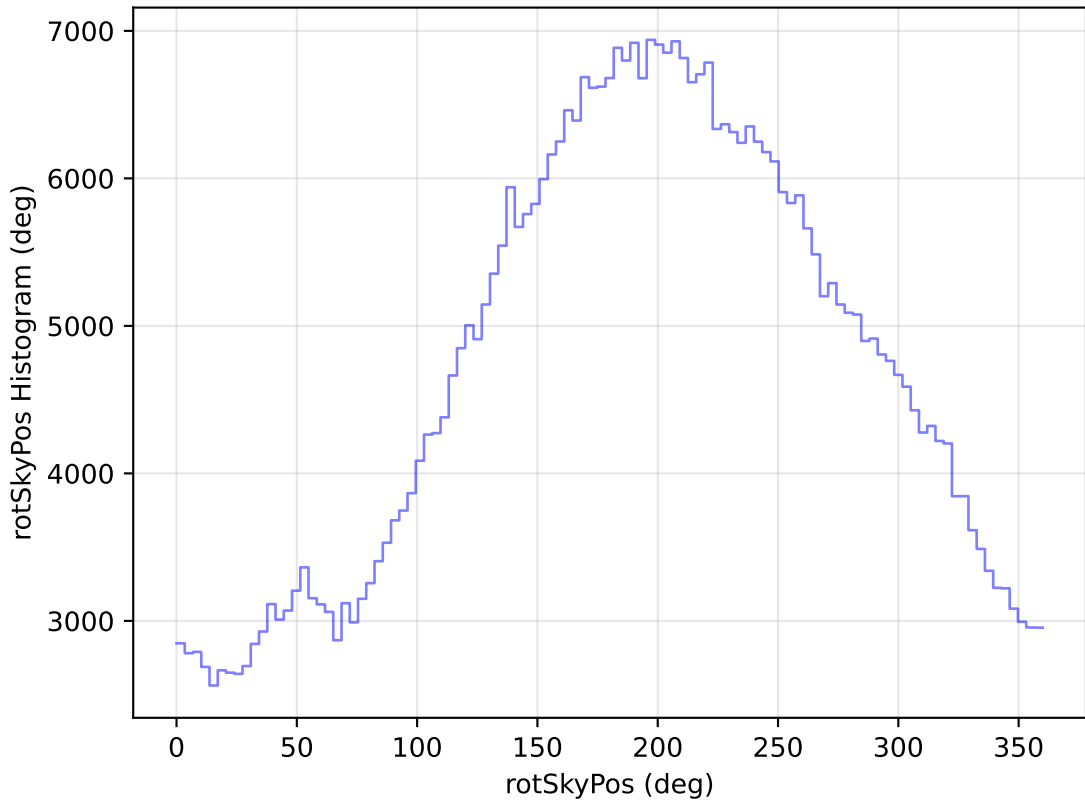
internal_u_expt27_nscale0.9v3.4_10yrs WFD r band: rotSkyPos Histogram
