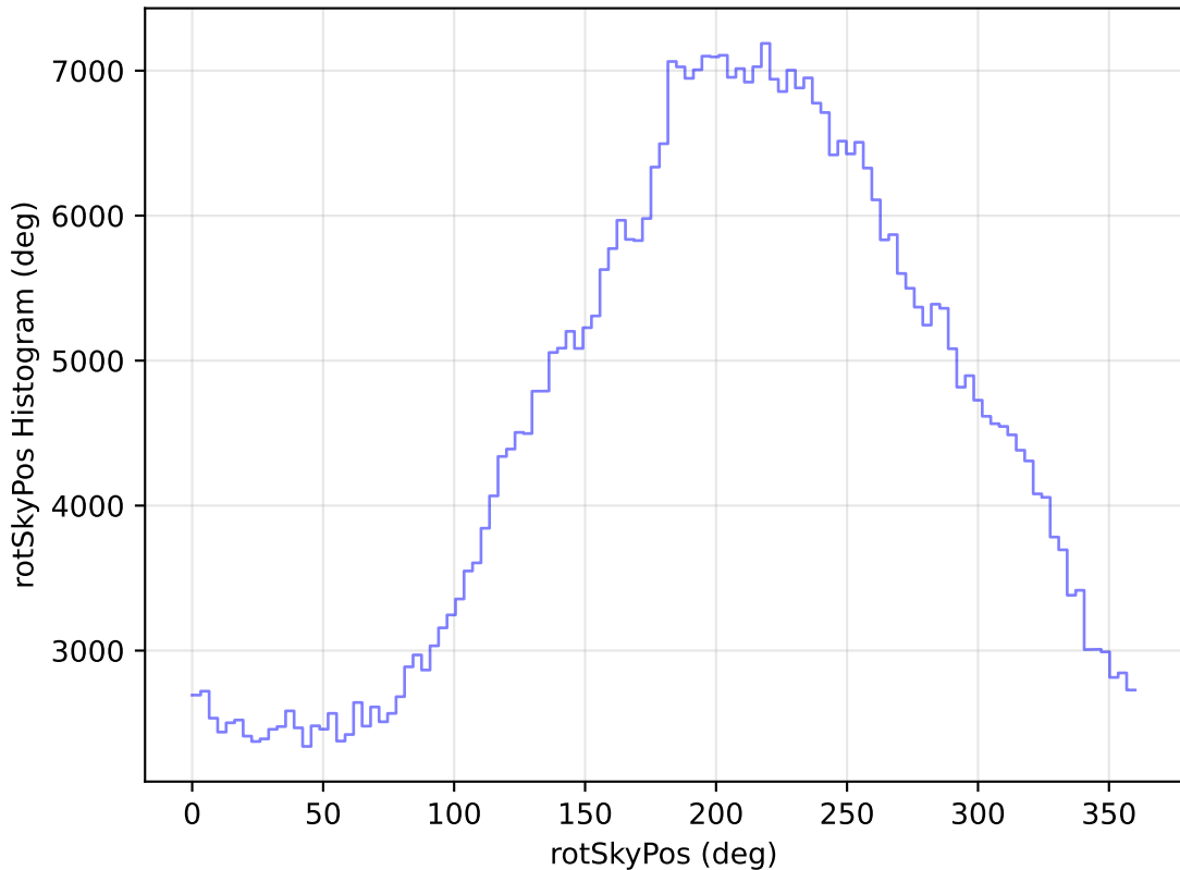
internal_u_expt27_nscale0.9v3.4_10yrs WFD i band: rotSkyPos Histogram
