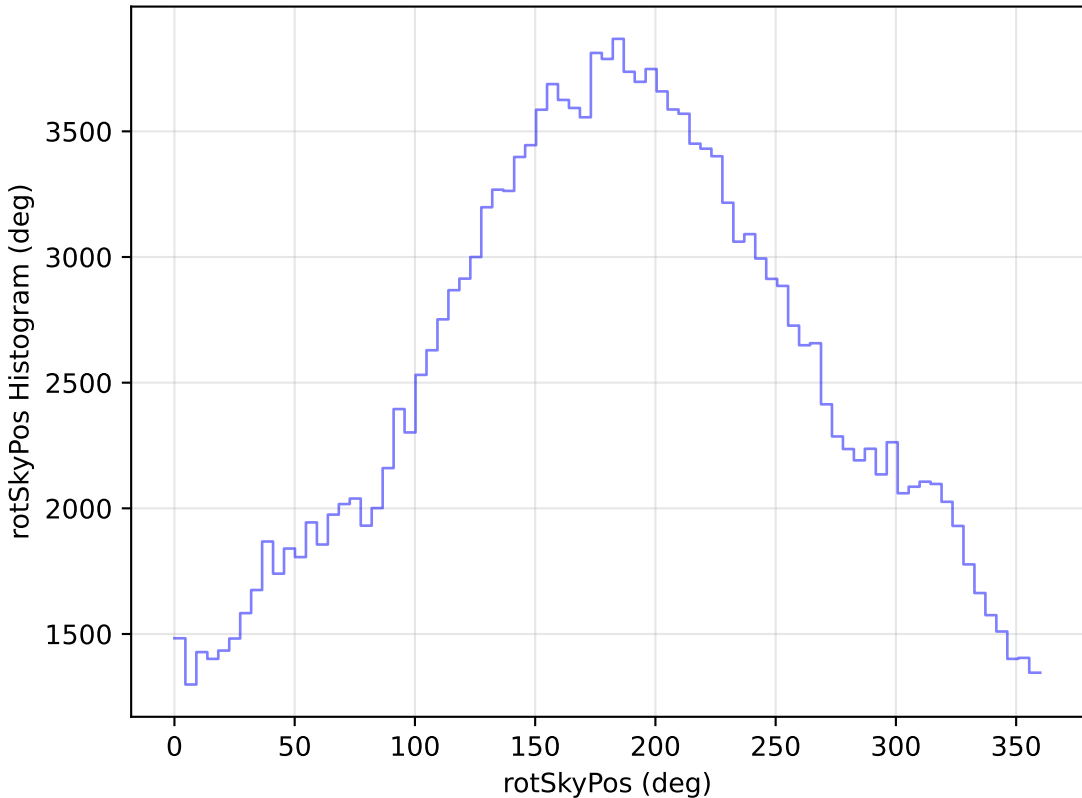
internal_u_expt27_nscale0.9v3.4_10yrs WFD g band: rotSkyPos Histogram
