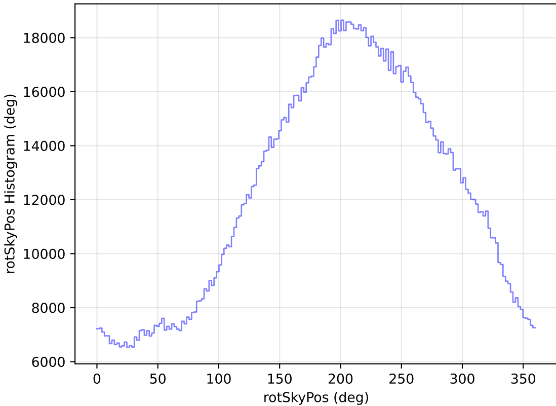
internal_u_expt27_nscale0.9v3.4_10yrs WFD all bands: rotSkyPos Histogram
