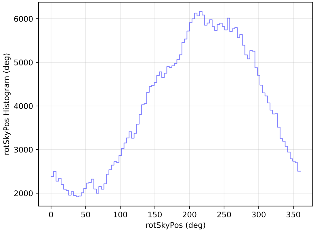
internal_u_expt27_nscale0.9v3.4_10yrs All sky y band: rotSkyPos Histogram
