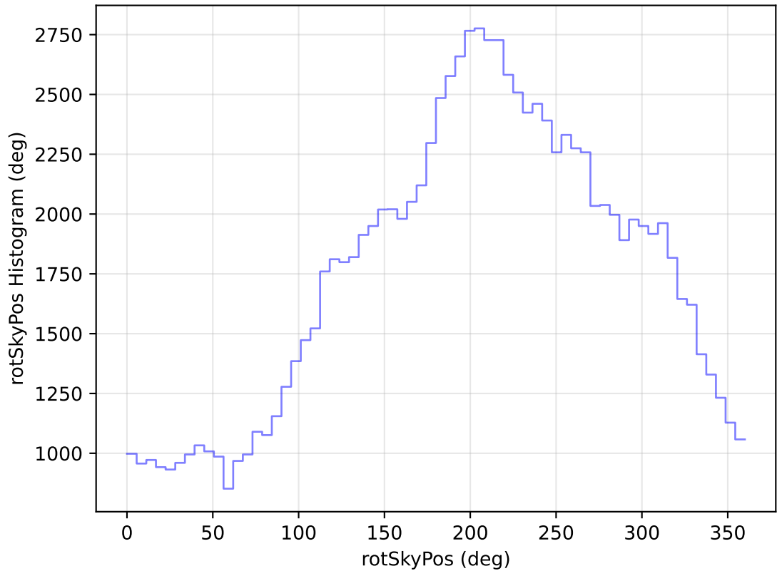
internal_u_expt27_nscale0.9v3.4_10yrs All sky u band: rotSkyPos Histogram
