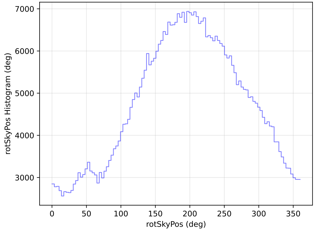
internal_u_expt27_nscale0.9v3.4_10yrs All sky r band: rotSkyPos Histogram
