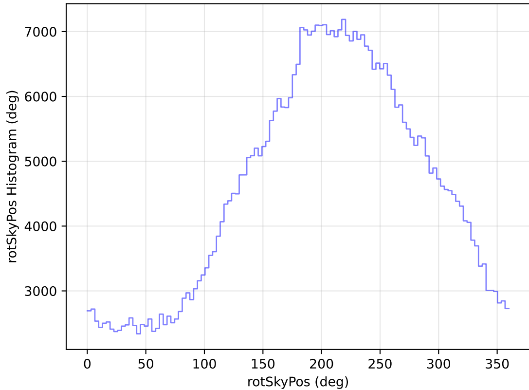
internal_u_expt27_nscale0.9v3.4_10yrs All sky i band: rotSkyPos Histogram
