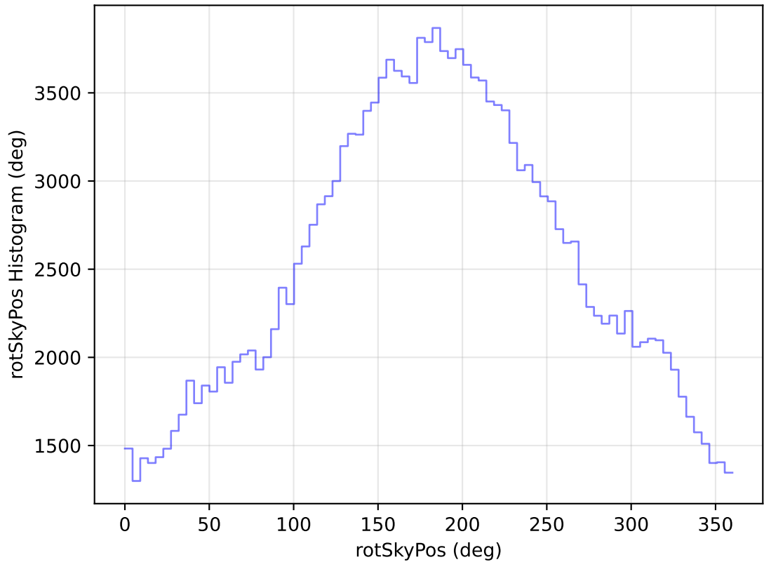
internal_u_expt27_nscale0.9v3.4_10yrs All sky g band: rotSkyPos Histogram
