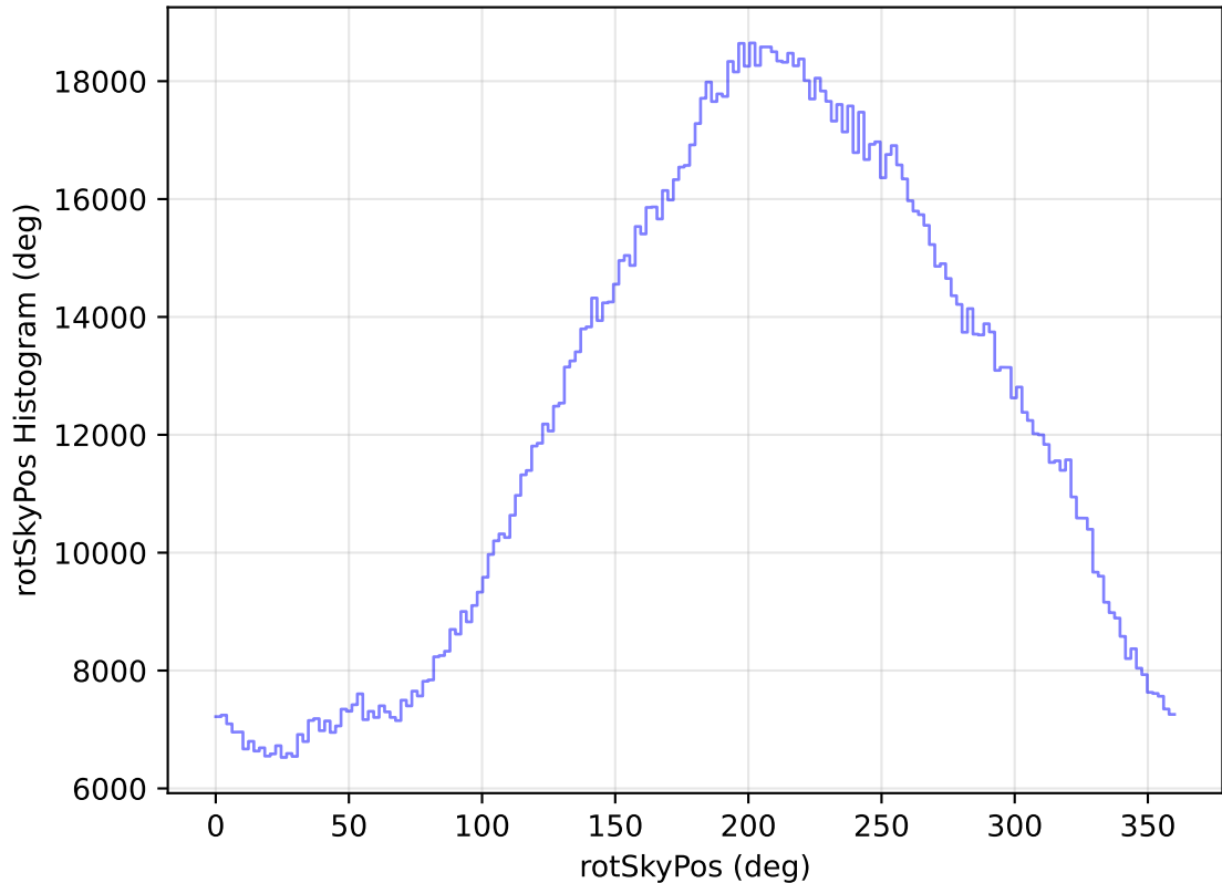
internal_u_expt27_nscale0.9v3.4_10yrs All sky all bands: rotSkyPos Histogram
