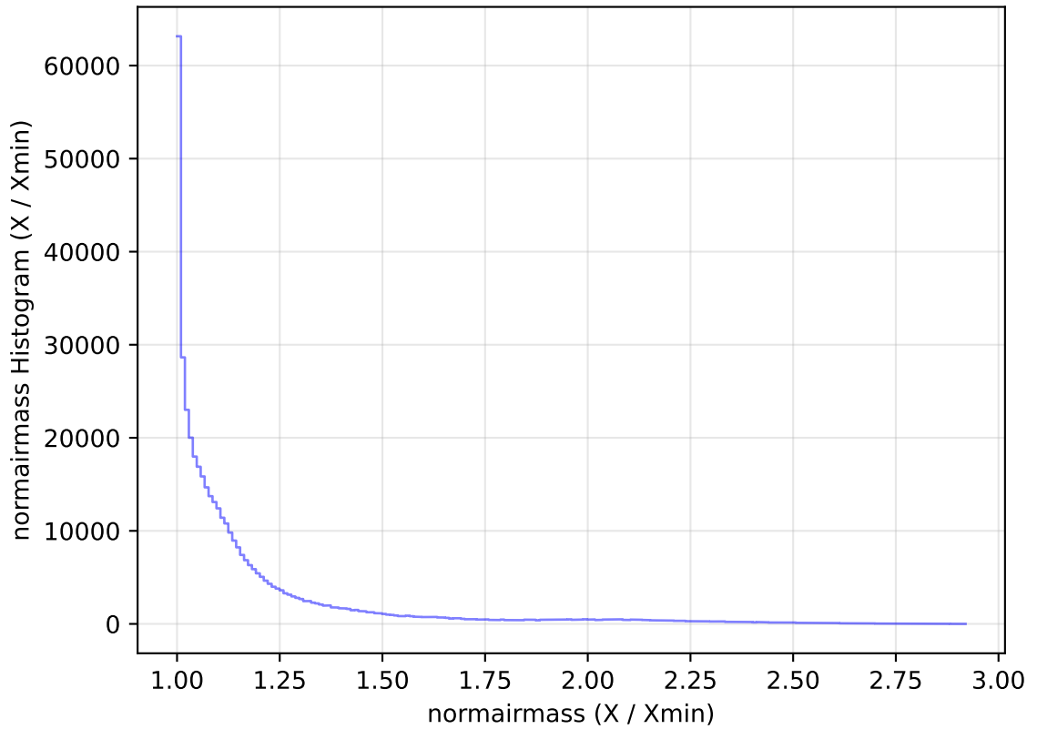
internal_u_expt27_nscale0.9v3.4_10yrs WFD z band: normairmass Histogram
