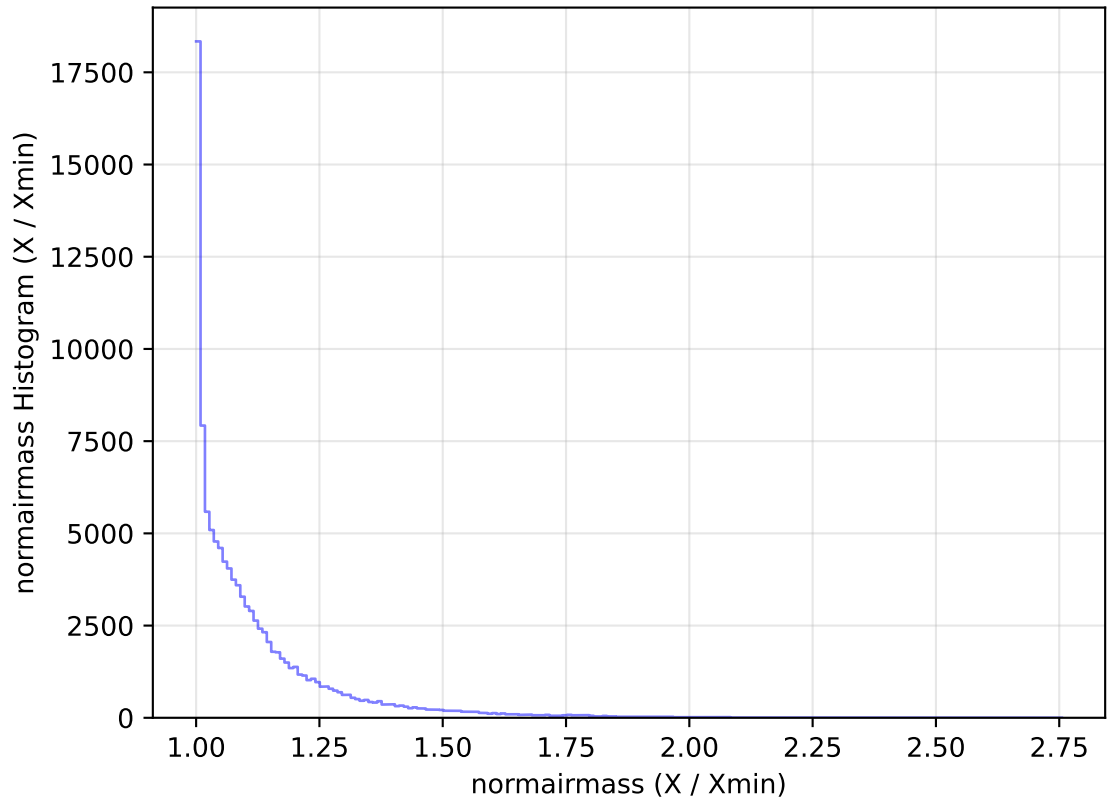
internal_u_expt27_nscale0.9v3.4_10yrs WFD u band: normairmass Histogram
