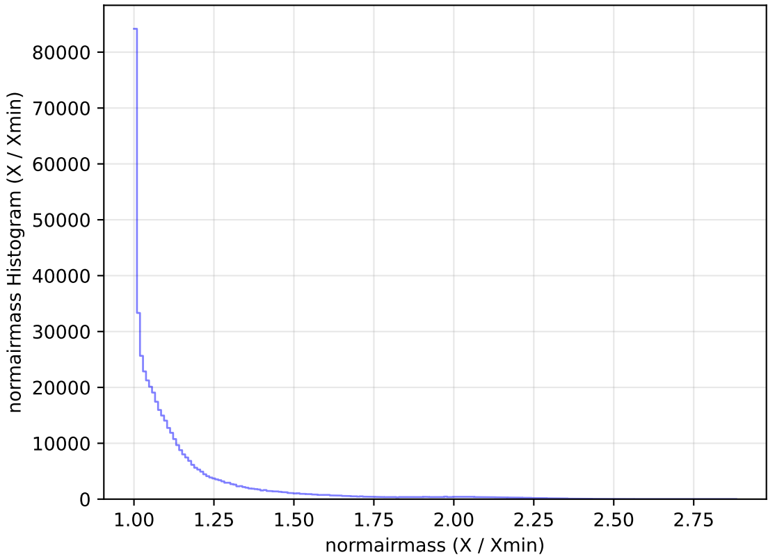
internal_u_expt27_nscale0.9v3.4_10yrs WFD r band: normairmass Histogram
