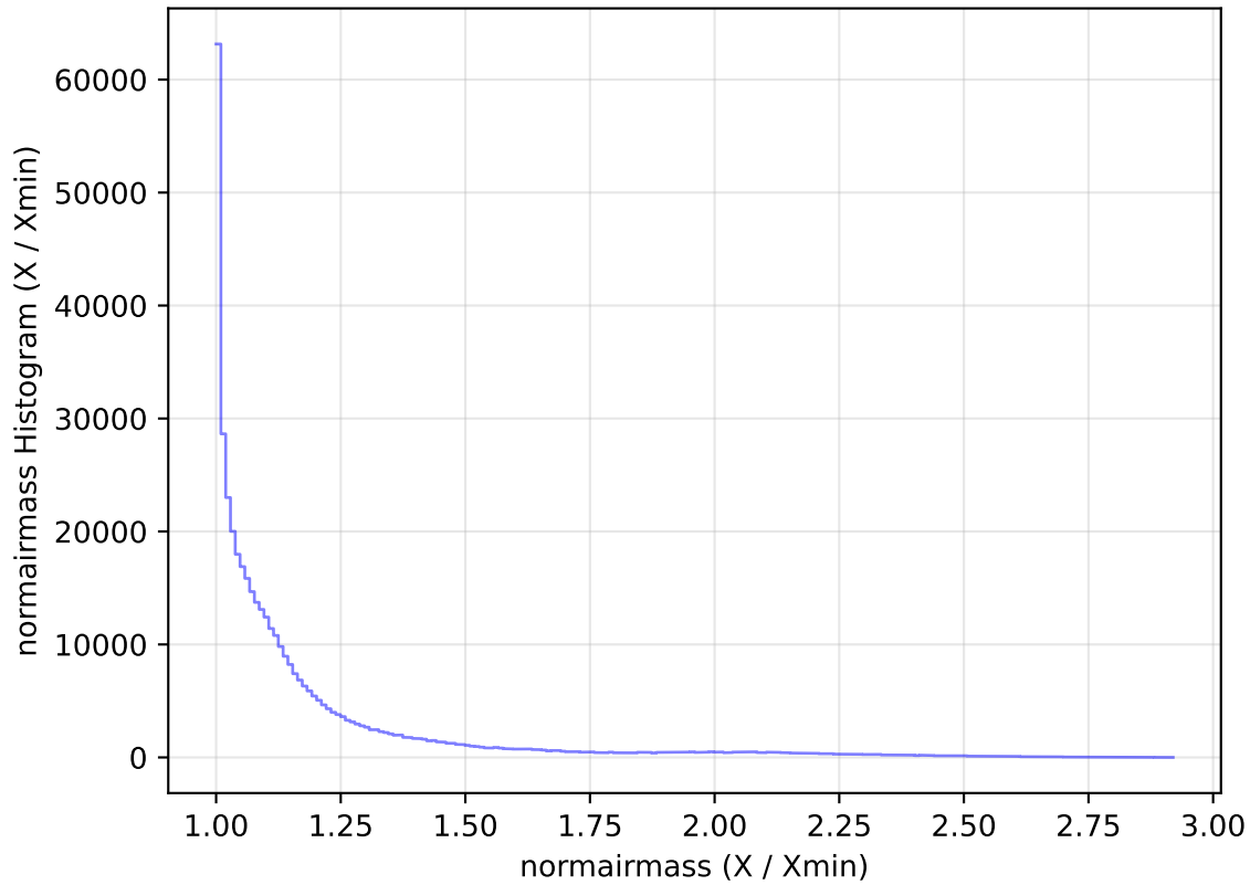
internal_u_expt27_nscale0.9v3.4_10yrs All sky z band: normairmass Histogram
