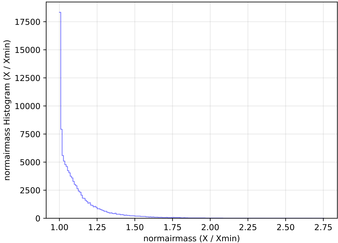
internal_u_expt27_nscale0.9v3.4_10yrs All sky u band: normairmass Histogram
