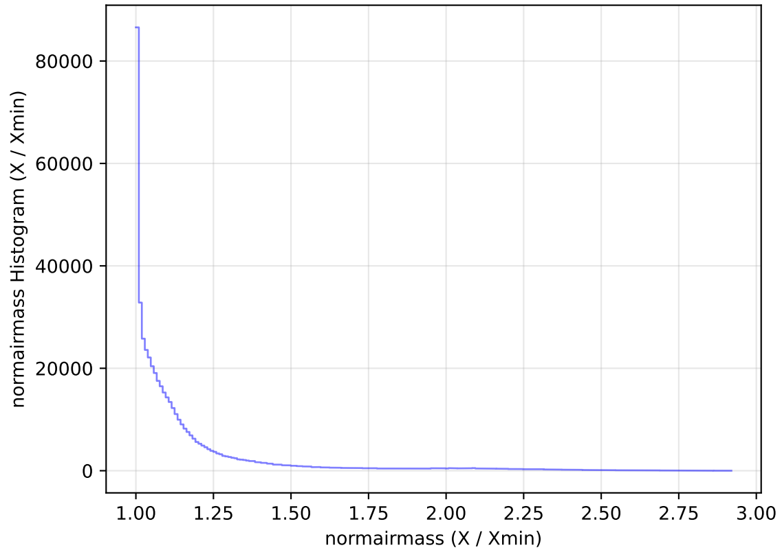
internal_u_expt27_nscale0.9v3.4_10yrs All sky i band: normairmass Histogram
