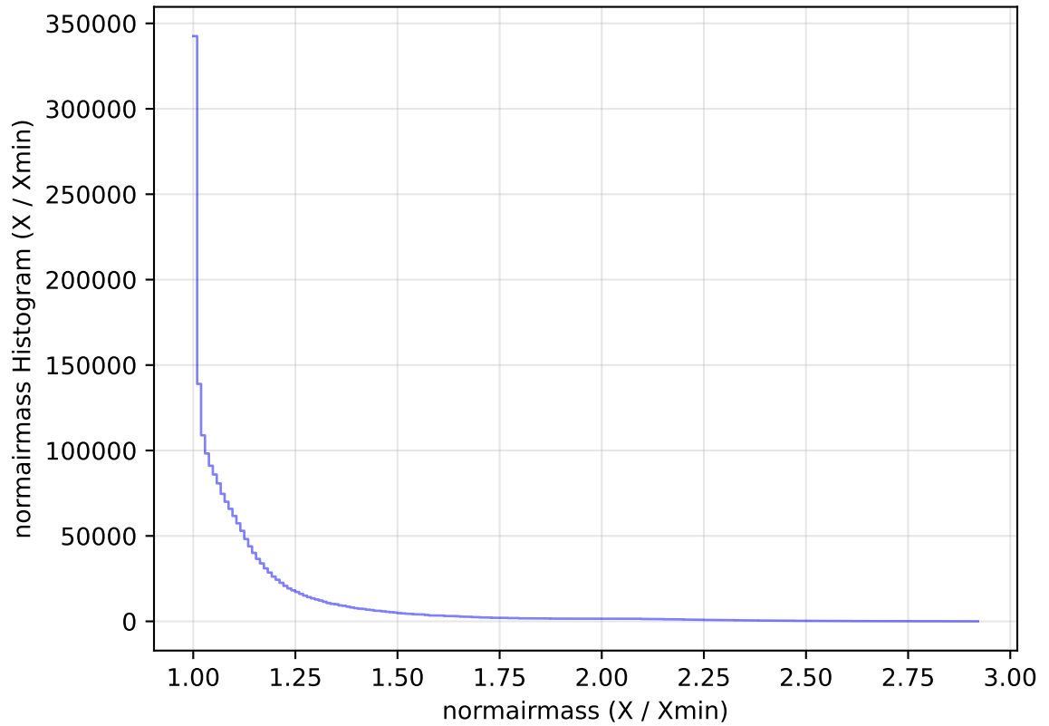
internal_u_expt27_nscale0.9v3.4_10yrs All sky all bands: normairmass Histogram
