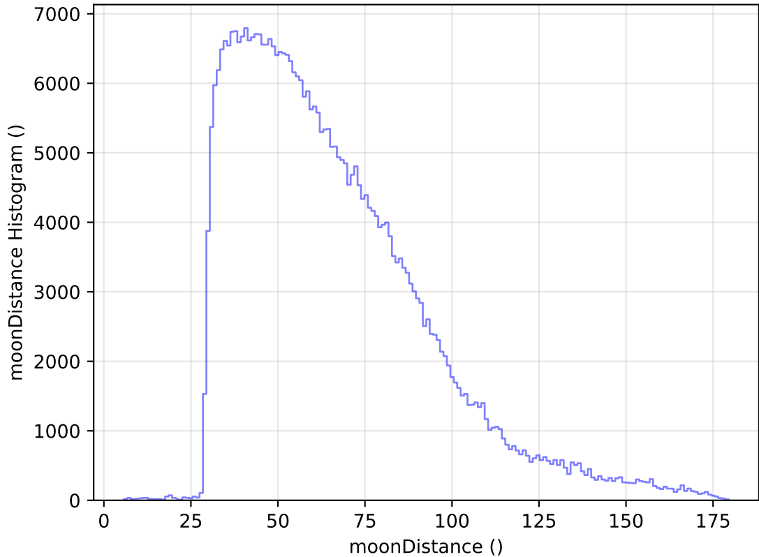
internal_u_expt27_nscale0.9v3.4_10yrs WFD y band: moonDistance Histogram
