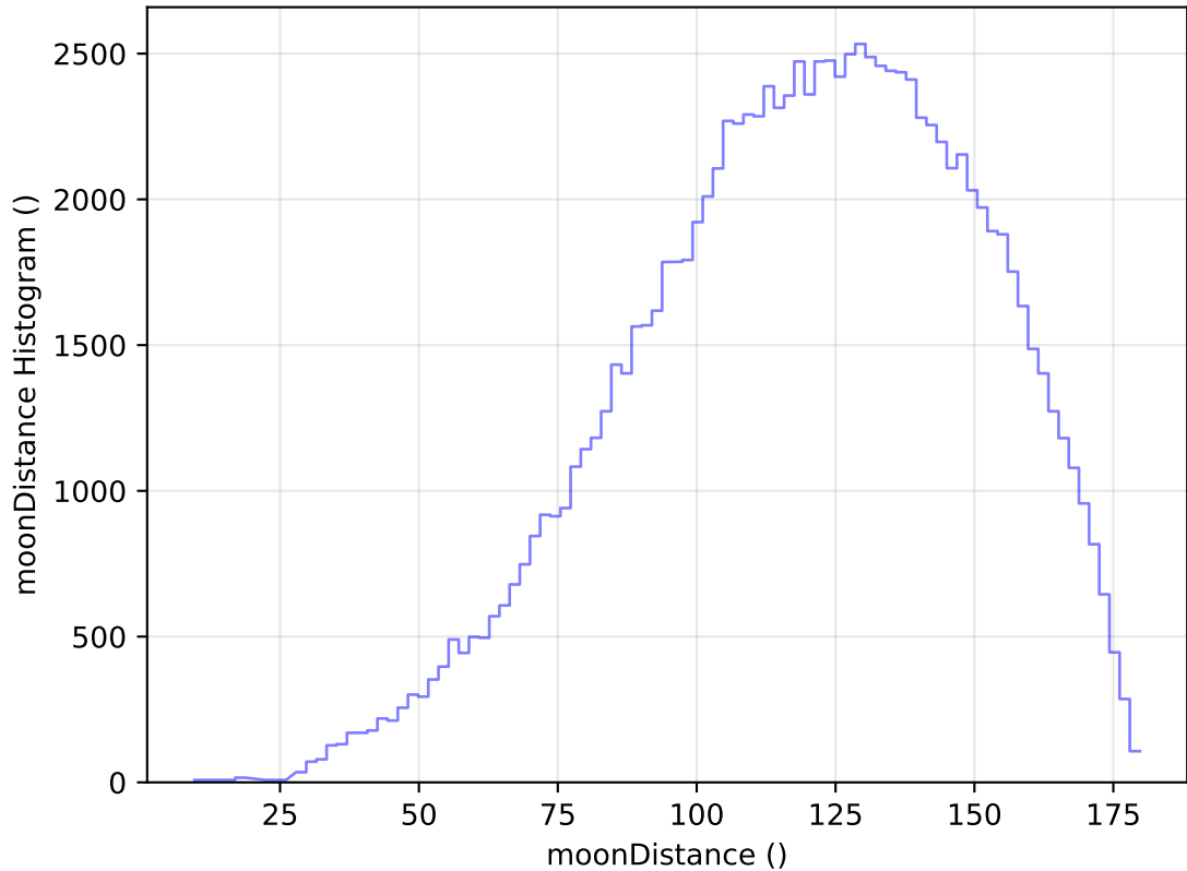
internal_u_expt27_nscale0.9v3.4_10yrs WFD u band: moonDistance Histogram
