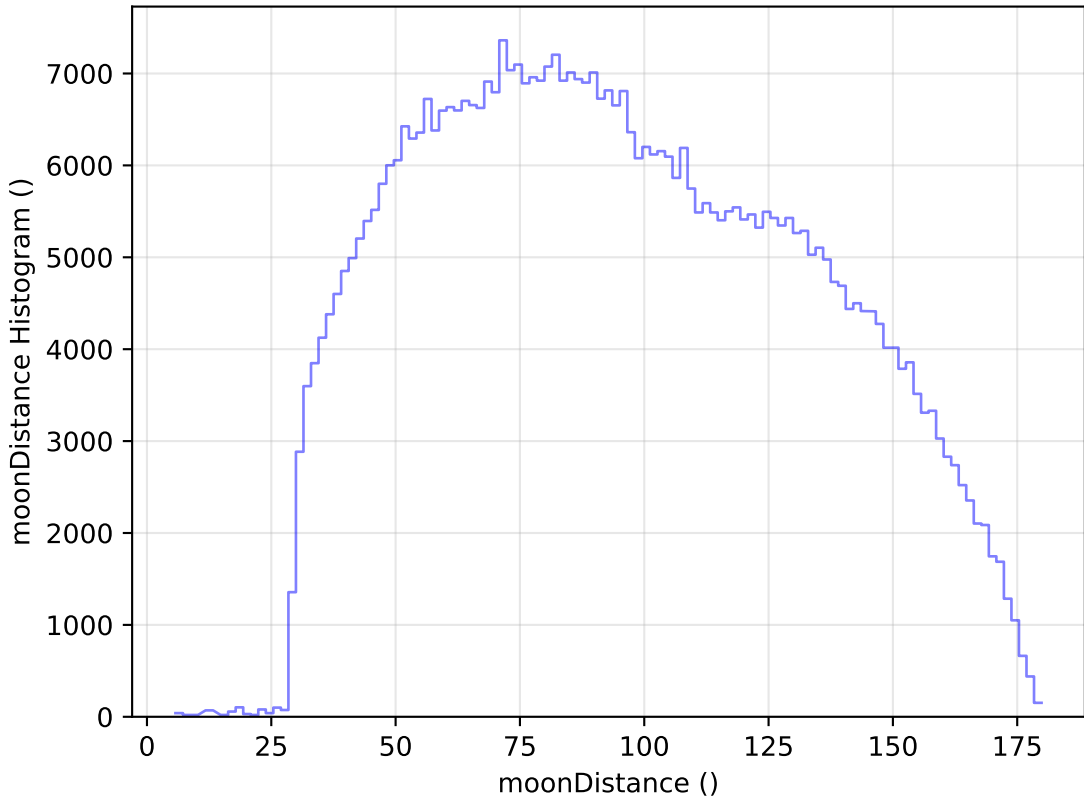
internal_u_expt27_nscale0.9v3.4_10yrs WFD i band: moonDistance Histogram
