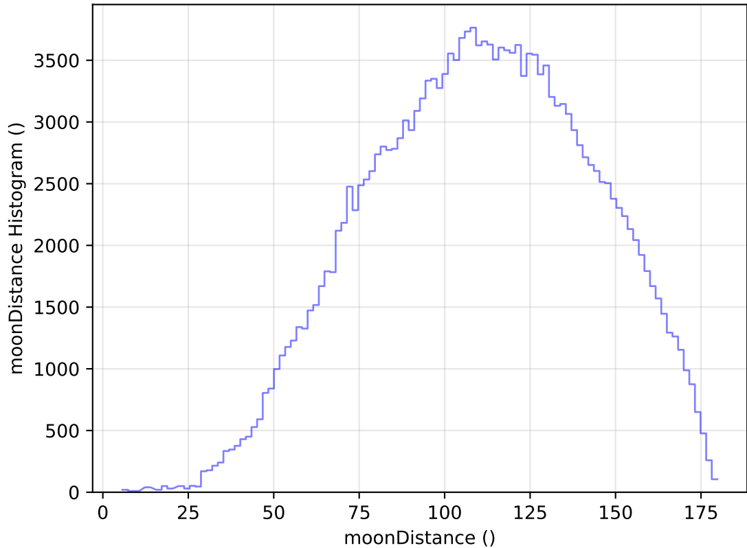
internal_u_expt27_nscale0.9v3.4_10yrs WFD g band: moonDistance Histogram
