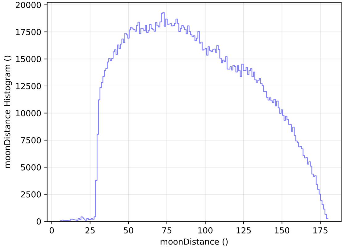
internal_u_expt27_nscale0.9v3.4_10yrs WFD all bands: moonDistance Histogram
