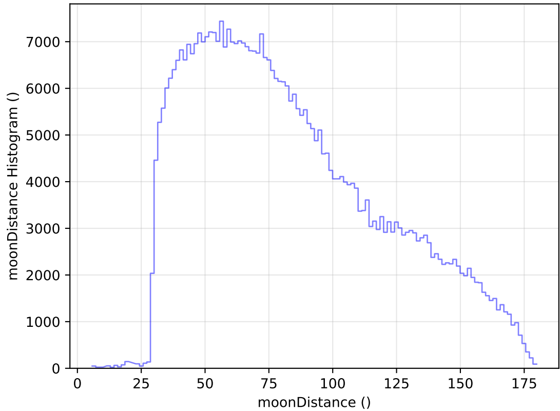
internal_u_expt27_nscale0.9v3.4_10yrs All sky z band: moonDistance Histogram
