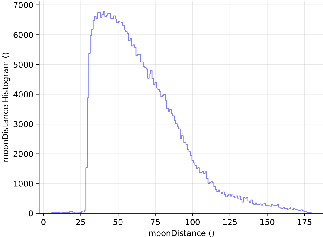
internal_u_expt27_nscale0.9v3.4_10yrs All sky y band: moonDistance Histogram
