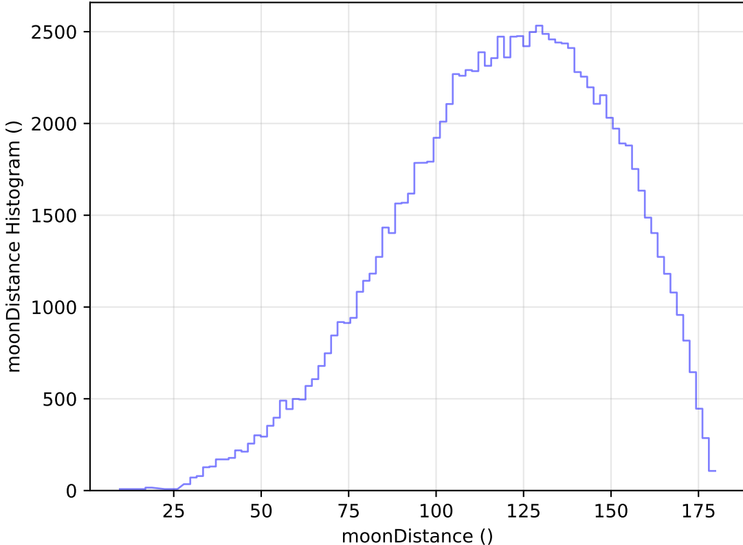
internal_u_expt27_nscale0.9v3.4_10yrs All sky u band: moonDistance Histogram
