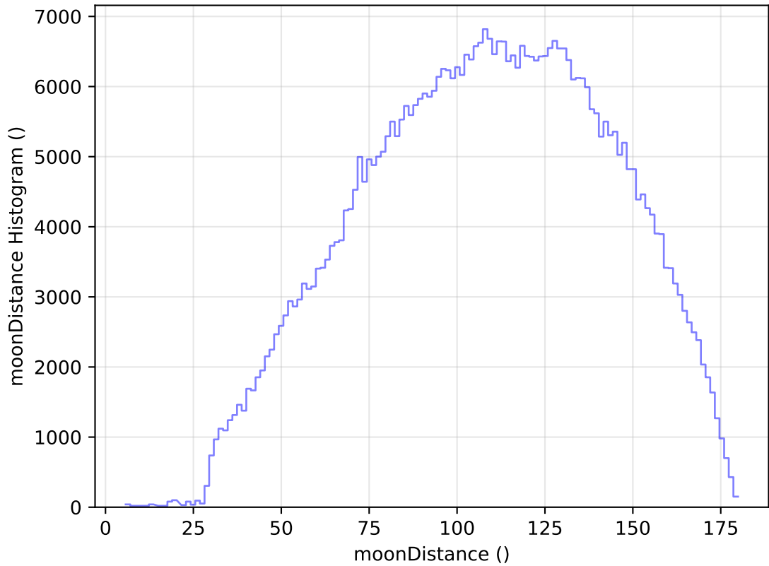
internal_u_expt27_nscale0.9v3.4_10yrs All sky r band: moonDistance Histogram
