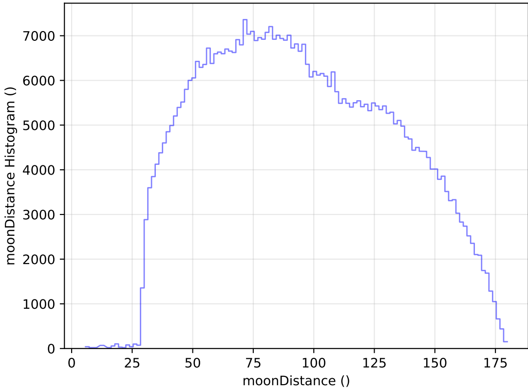
internal_u_expt27_nscale0.9v3.4_10yrs All sky i band: moonDistance Histogram
