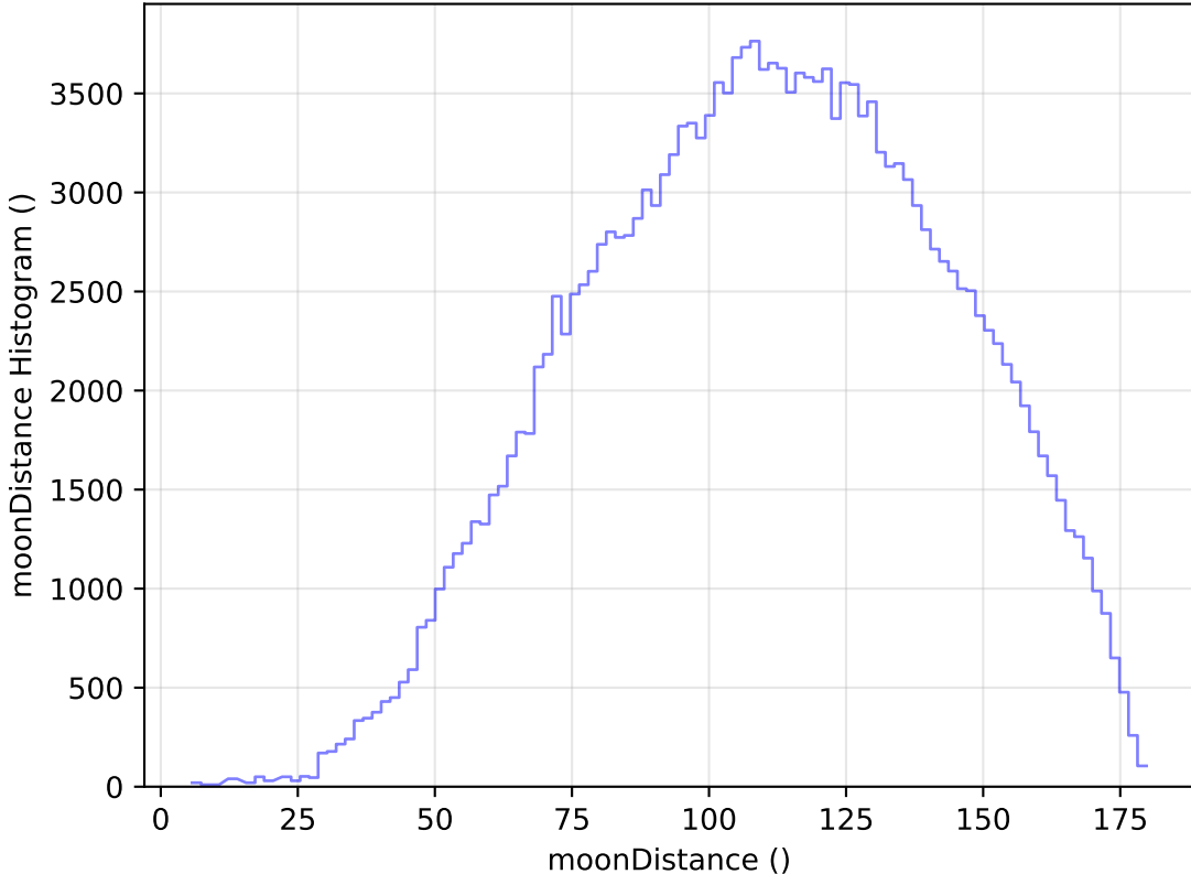
internal_u_expt27_nscale0.9v3.4_10yrs All sky g band: moonDistance Histogram
