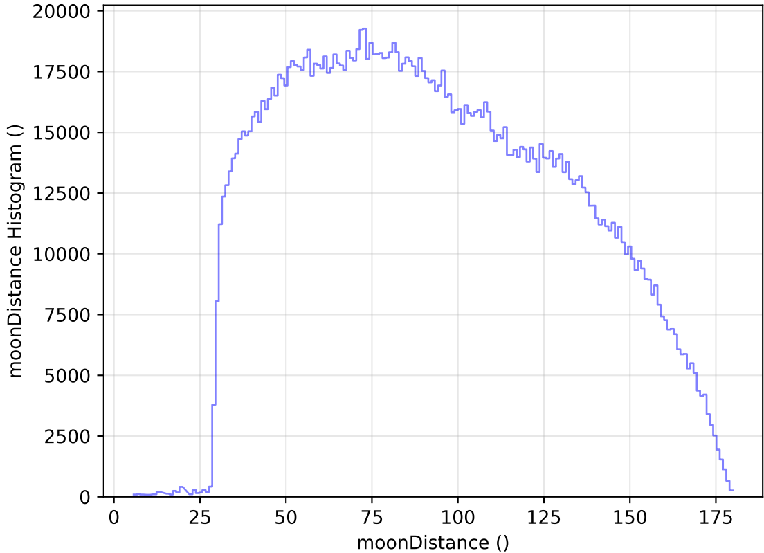
internal_u_expt27_nscale0.9v3.4_10yrs All sky all bands: moonDistance Histogram
