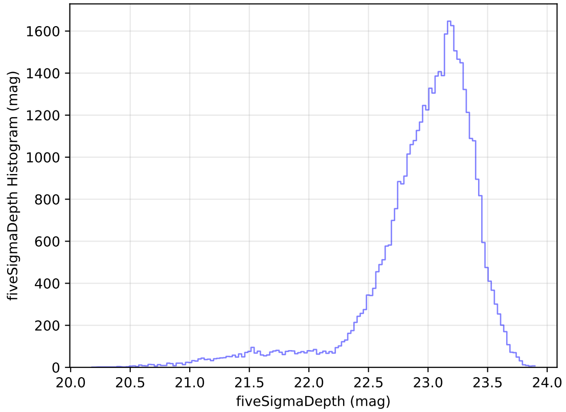
internal_u_expt27_nscale0.9v3.4_10yrs Yr 1 z band: fiveSigmaDepth Histogram
