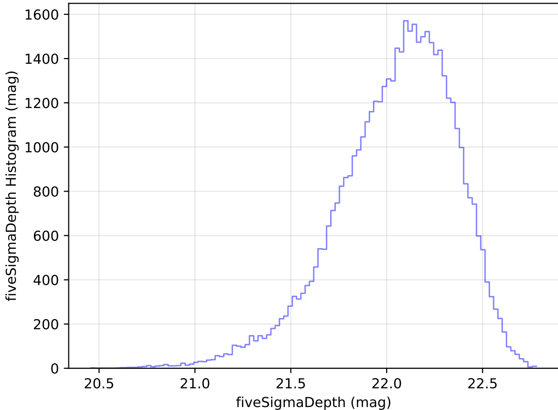
internal_u_expt27_nscale0.9v3.4_10yrs Yr 1 y band: fiveSigmaDepth Histogram
